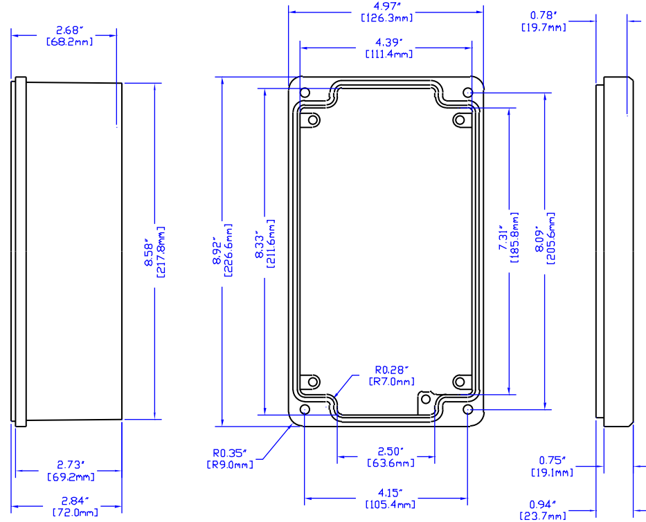
VIEW OF LID (INSIDE)
