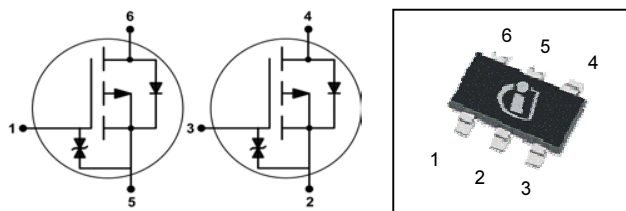
PG-TSOP-6
