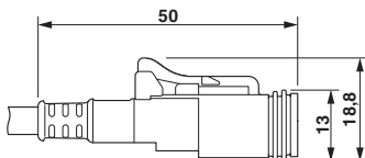
Dimensional drawing
