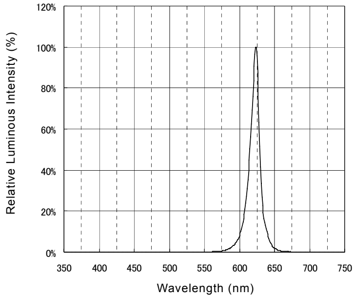
Relative Luminous Intensity — Wavelength Characteristics
