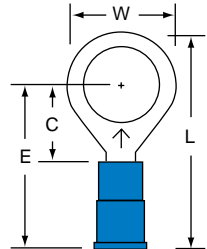
MVU14-38R Stud Size 3/8 Wire Range 16-14
