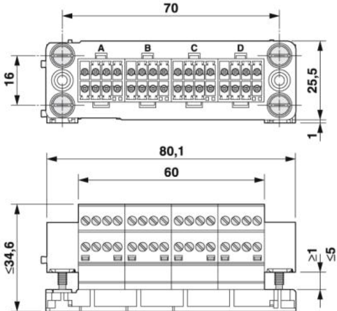
Dimensional drawing
