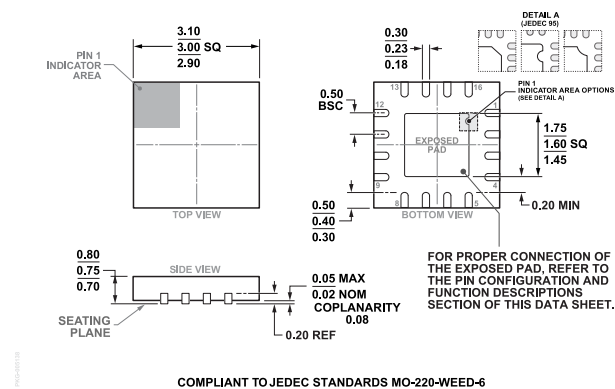
Figure 50. 16-Lead Frame Chip Scale Package [LFCSP] 3 mm × 3 mm Body and 0.75 mm Package Height (CP-16-22) Dimensions shown in millimeters
