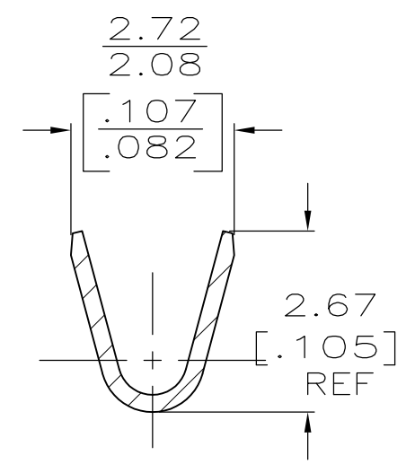
SECTION X-X SCALE 10:1
