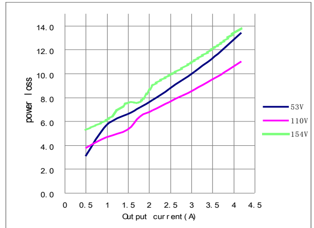
Figure 2: Power dissipation vs. load current for 53, 110 and 154 input voltage at 25°C.
