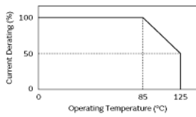
Derating of Rated Current
