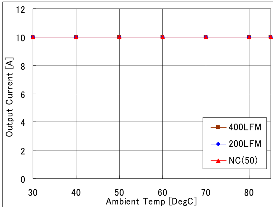
Fig-1.2V-1: Available load current vs. ambient temperature and airflow rates for V_{out}=1.2V with V_{in}=12.0V . Maximum component temperature \leq 120^{\circ}C
