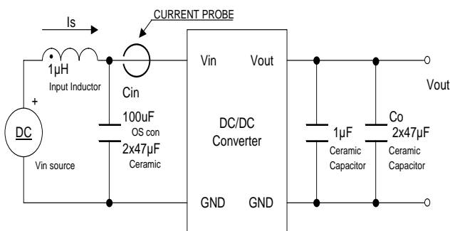
Fig. J: Test setup for measuring input reflected ripple current
