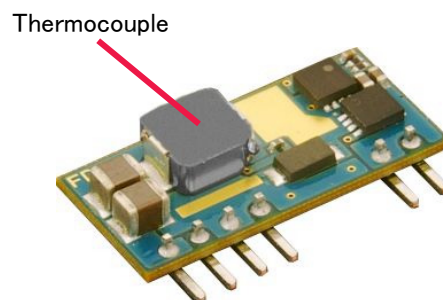
Fig. H: Location of the thermocouples for thermal testing
