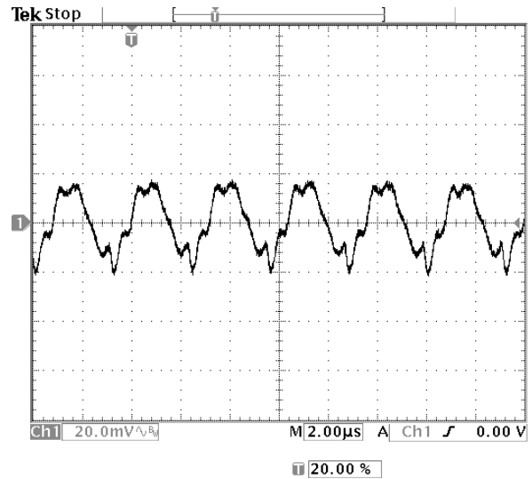
Fig-5.0V-5: Output voltage ripple (20mV/div.) for V_{out}=5.0V at full rated load current into a resistive load with external capacitance 47\mu F \times 2 ceramic + 1\mu F ceramic at V_{in}=12.0V .
