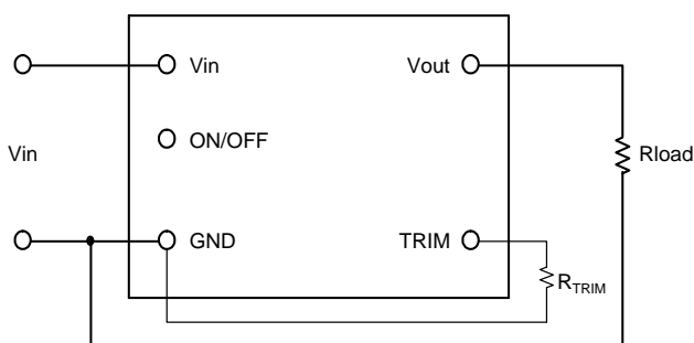
Fig.B: Configuration for programming output voltage
