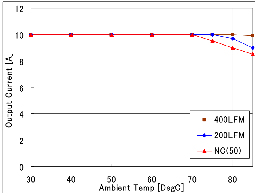
Fig-5.0V-1: Available load current vs. ambient temperature and airflow rates for V_{out}=5.0V with V_{in}=12.0V . Maximum component temperature \leq 120^{\circ}C
