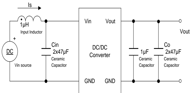
Fig. I: Test setup for measuring output voltage ripple
