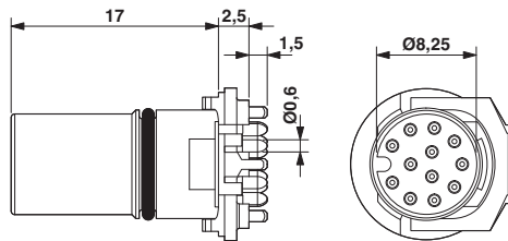
M12 socket, straight
