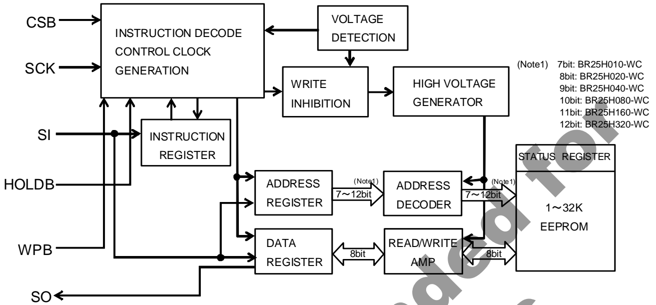
Figure 4. Block diagram
