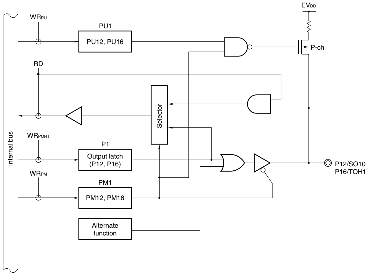
Figure 4-6. Block Diagram of P12 and P16
