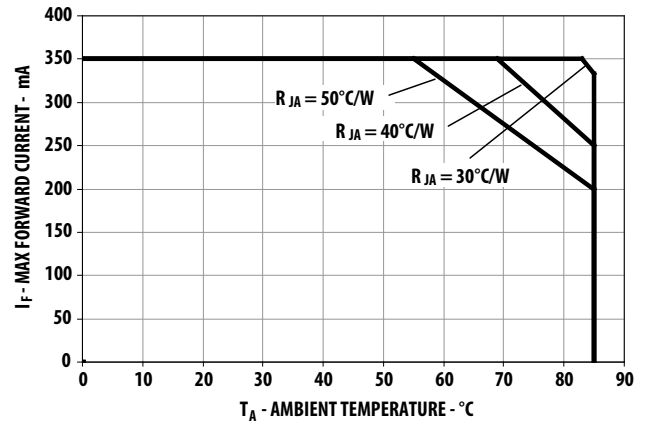
Figure 8. Maximum forward current vs. ambient temperature Derated based on T_{JMAX} = 125^{\circ}C , R_{\theta JA} = 30^{\circ}C/W , 40^{\circ}C/W and 50^{\circ}C/W
