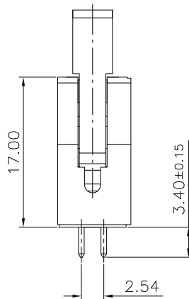
MATING PART 3030-XX-0101-00
