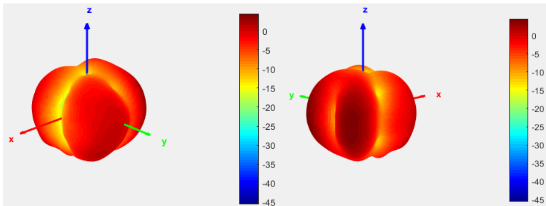
Radiation Pattern @ 9GHz
