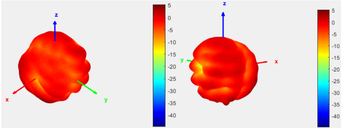
Radiation Pattern @ 3GHz
