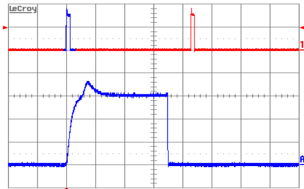
Figure 15. Load current (top trace, 20 A/div., 50 ms/div.) into a 10 mΩ short circuit during restart, at V_{in} = 48 V . Bottom trace (10 A/div., 2ms/div.) is an expansion of the on-time portion of the top trace.
