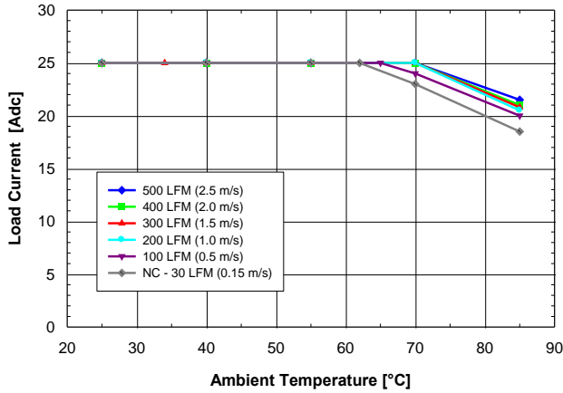
Figure 1. Available load current vs. ambient air temperature and airflow rates for SSQE48T25015 converter mounted vertically with air flowing from pin 1 to pin 3, Vin = 48V. Note: NC - Natural convection
