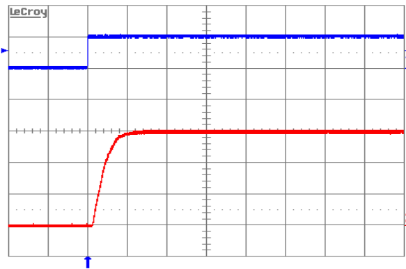
Figure 7. Turn-on transient at full rated load current (resistive) plus 30,000µF at V_{in} = 48\text{ V} , triggered via ON/OFF pin. Top trace: ON/OFF signal (5 V/div.). Bottom trace: Output voltage (0.5 V/div.). Time scale: 5 ms/div.
