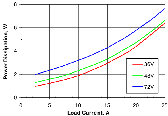
Figure 4. Power dissipation vs. load current and input voltage for SSQE48T25015 converter mounted vertically with air flowing from pin 1 to pin 3 at a rate of 300 LFM (1.5 m/s) and Ta = 25 °C.
