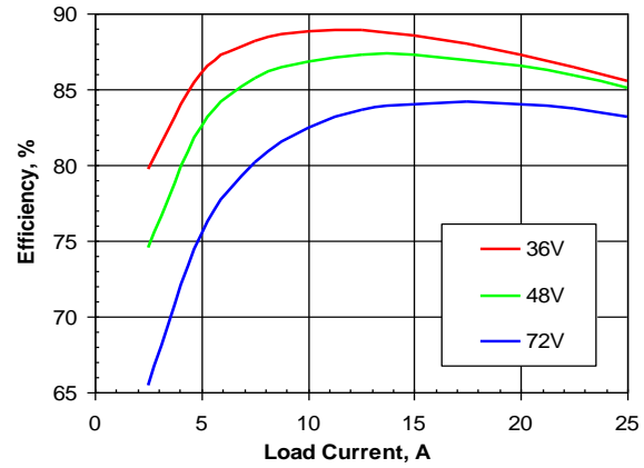
Figure 2. Efficiency vs. load current and input voltage for SSQE48T25015 converter mounted vertically with air flowing from pin 1 to pin 3 at a rate of 300 LFM (1.5 m/s) and Ta=25°C.
