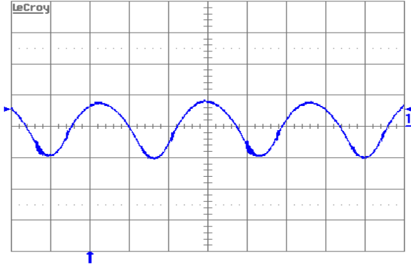
Figure 13. Input reflected ripple-current, i_c (200 mA/div.), measured at input terminals at full rated load current and V_{in} = 48 V . Refer to Figure 11 for test setup. Time scale: 1 μs/div.
