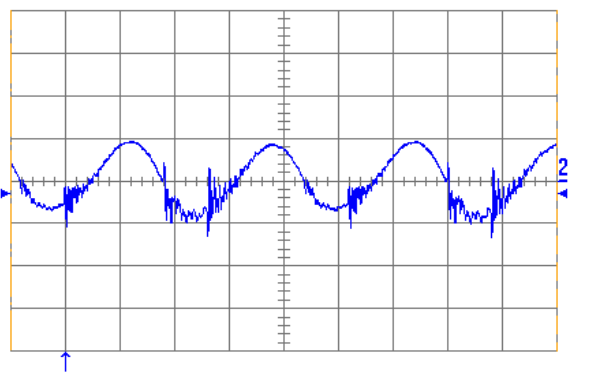
Figure 10. Output voltage ripple (20mV/div.) at full rated load current into a resistive load with C_o = 10\mu\text{F tantalum} + 1\mu\text{F ceramic} and V_{in} = 48\text{ V} . Time scale: 1µs/div.
