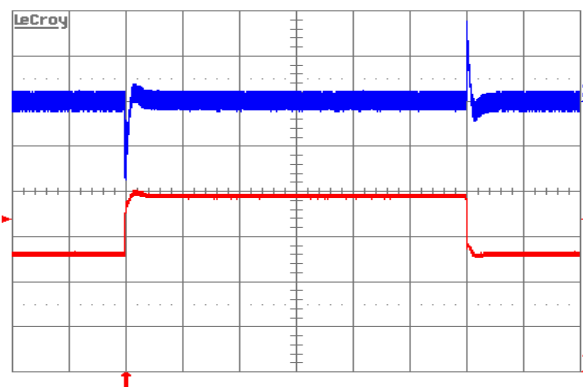
Figure 9. Output voltage response to load current step-change (12.5A–18.75A–12.5A) at V_{in} = 48\text{ V} . Top trace: output voltage (100 mV/div.). Bottom trace: load current (5A/div.). Current slew rate: 5A/µs. C_o = 470\mu\text{F POS} + 1\mu\text{F cer} . Time scale: 0.2ms/div.
