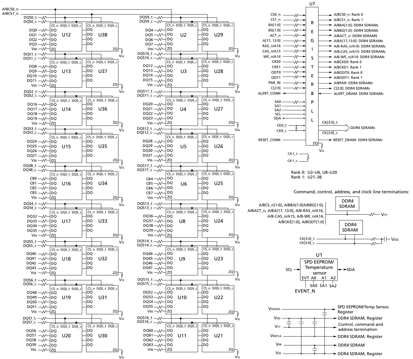
Figure 4: Functional Block Diagram, R/C-B2 (PCBs 1971, 2436, or 2615)
