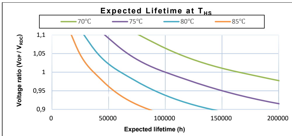
Service life t_{LD} in hours at different hotspot temperature ( T_{hs} ) and voltage V_{RDC} for \varnothing \leq 116 mm
