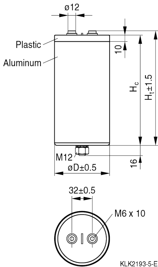
Figure 1: - B25690A – \varnothing = 75/85 mm - Female terminals (M6) - Between terminals 32 \pm 0.5 mm
