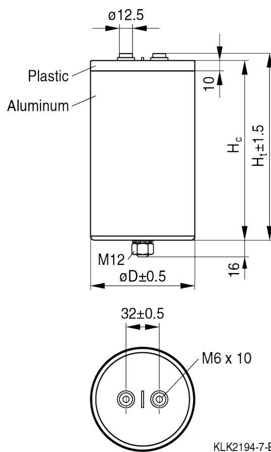
Figure 2: - B25690A – \varnothing = 100 mm - Female terminals (M6) - Between terminals 32 \pm 0.5 mm
