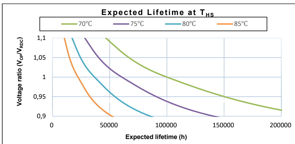
Service life t_{LD} in hours at different hotspot temperature ( T_{hs} ) and voltage V_{RDC} for \varnothing = 136 mm
