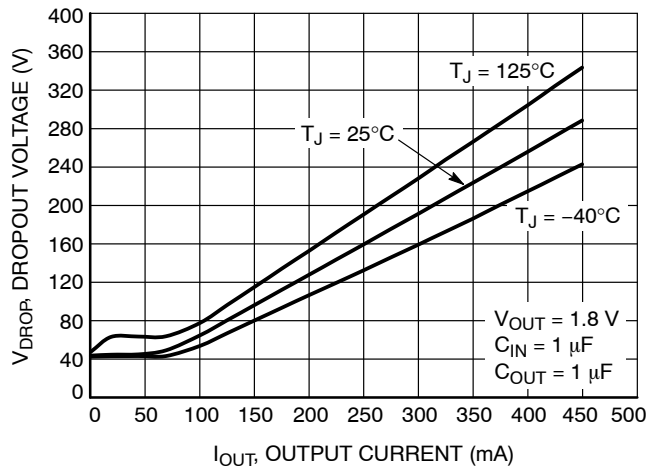
Figure 12. Dropout Voltage vs. Load Current - V_{OUT} = 1.8 V
