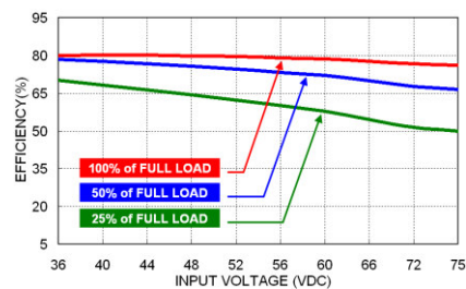
MPS(H)04-48S05 Efficiency vs. Input Voltage
