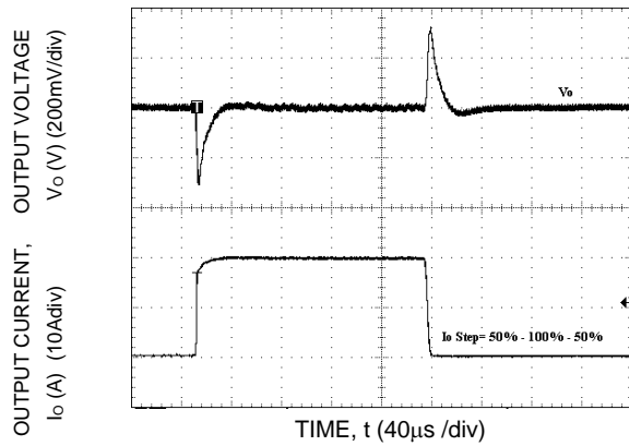
Figure 28. Transient Response to Dynamic Load Change from 0% to 50% to 100% to 0% with V_{IN}=12V .
