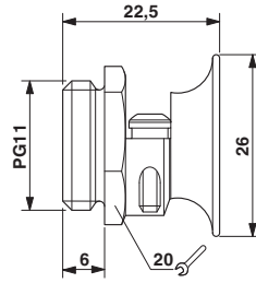
Dimensioned drawing
