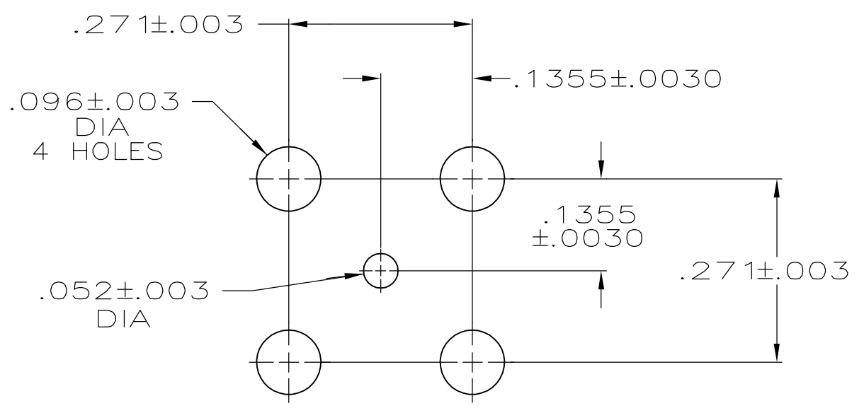
PCB CONFIGURATION
