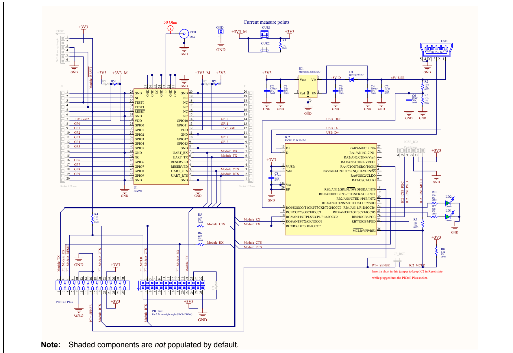
FIGURE A-1: RN2903 LoRa™ TECHNOLOGY PICtail™/PICtail PLUS DAUGHTER BOARD SCHEMATIC
