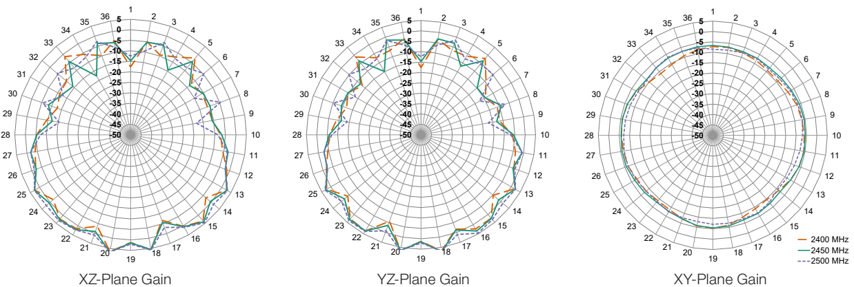
Figure 17. ANT-2.4-WRT Radiation Patterns
