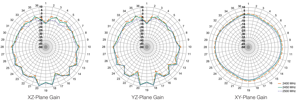
Figure 10. ANT-2.4-WRT Antenna Radiation Patterns, Free Space
