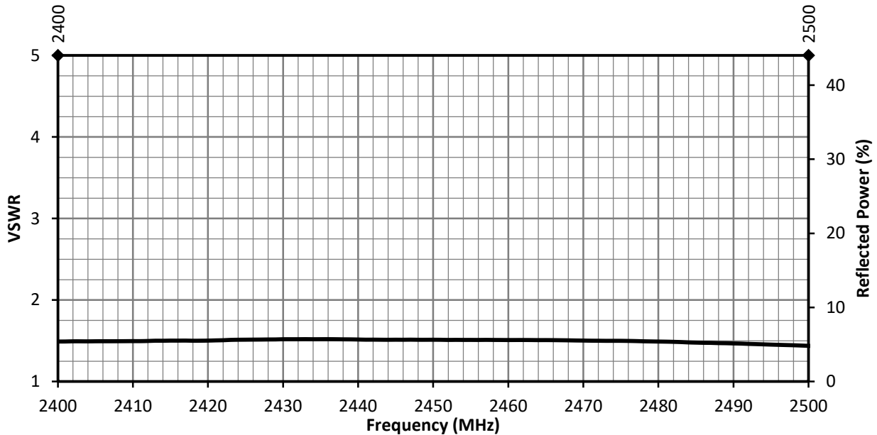
Figure 5. ANT-2.4-WRT VSWR, Free Space
