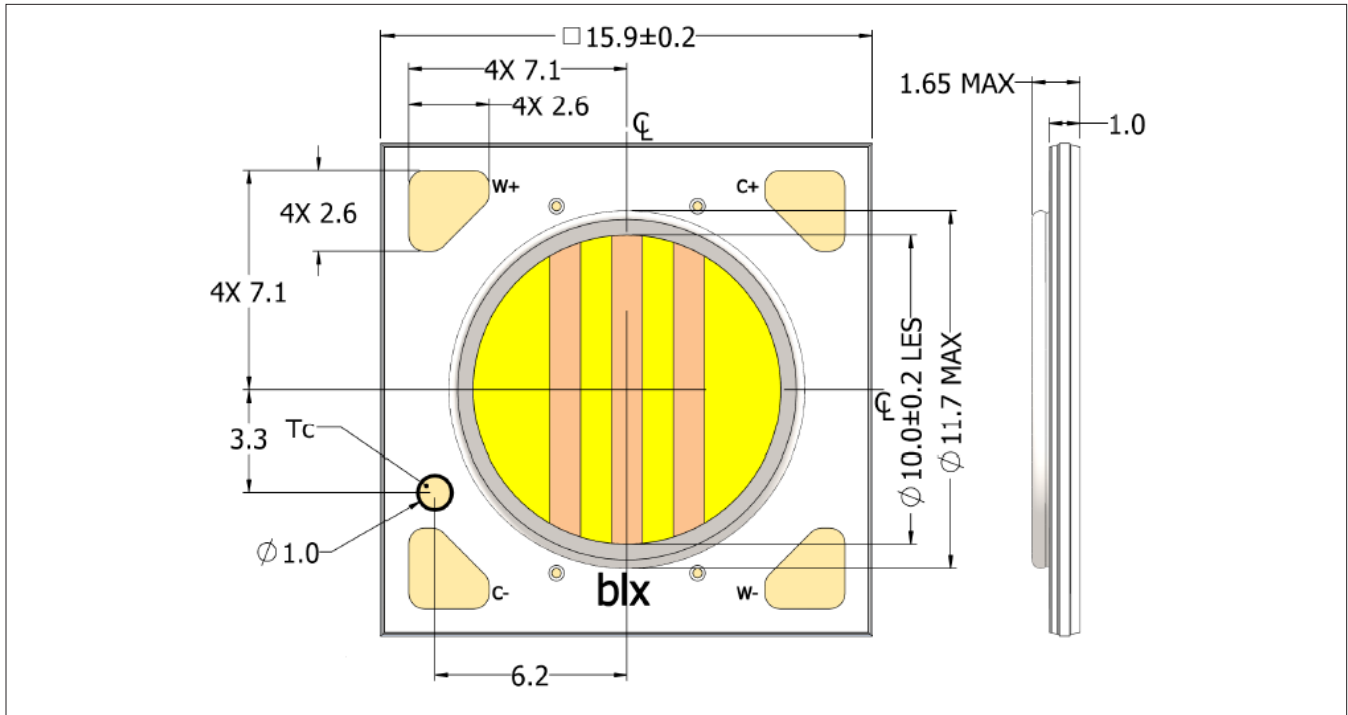
Figure 14: Drawing for Vesta Series Tunable White Gen2 9mm Array
