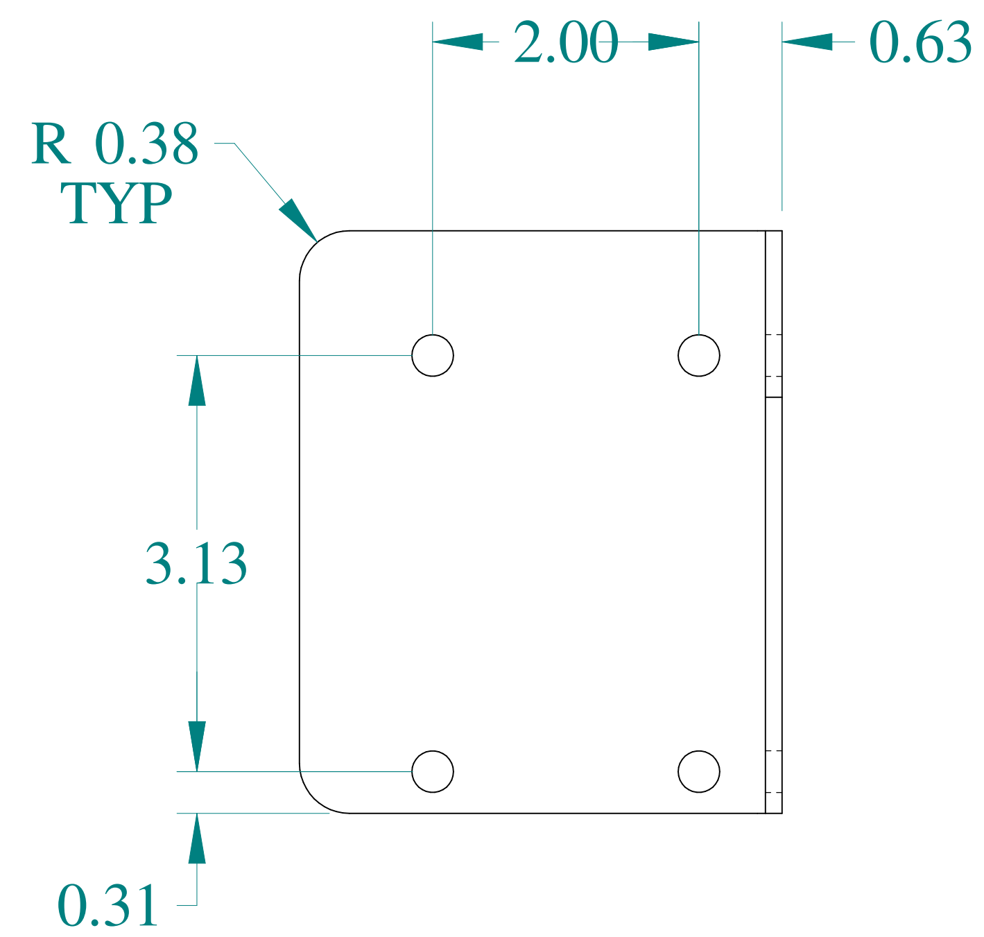
SIDE VIEW
