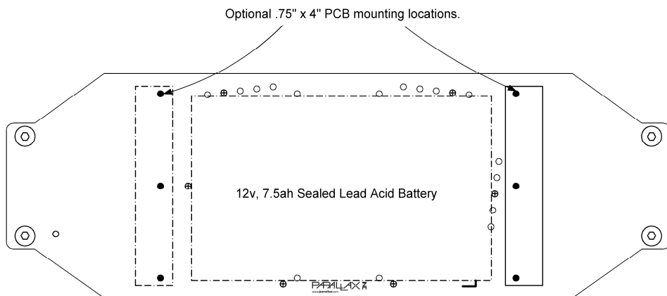
(As viewed from the bottom of Robot Base)
