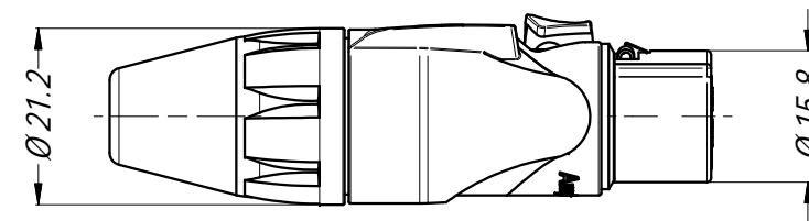
FEMALE CONNECTOR 1:1
