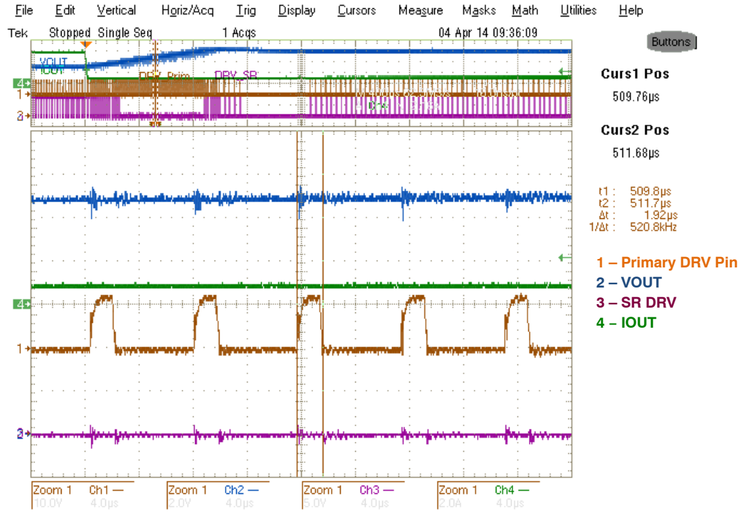
Figure 32. V_{IN} = 230 V_{AC} , R_{OUT} = 1.5 \Omega to 10 \Omega – Detail Shows why SR is Not Turned On. It is Not Turned-on, because Primary On-time is Shorter than Secondary Side Min-off Time (in CCM they Correspond Each Other)
