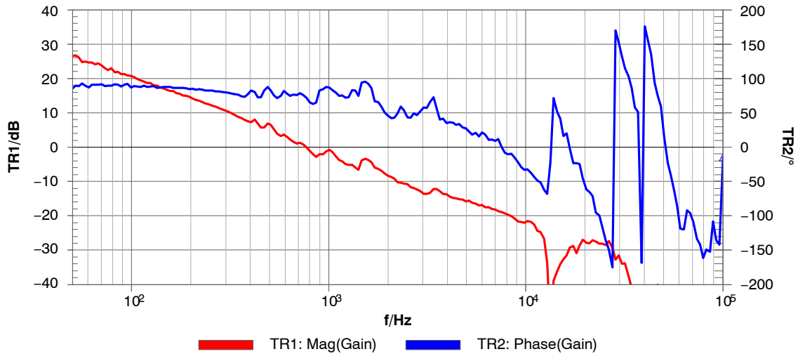
Figure 33. V_{IN} = 115 V_{AC} , I_{OUT} = 100 mA
