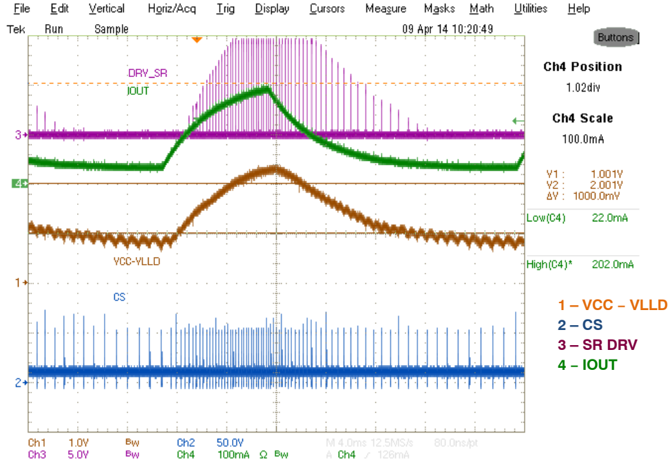
Figure 20. V_{IN} = 230\text{ V}_{AC} , I_{OUT} = 22\text{--}202\text{ mA} , SR Controller Driver Output Voltage is Modulated Accordingly to Load Current through LLD Pin. Regulation Range is 1 to 2 V. NCP4305 Enters Disable Mode where its Consumption Significantly Decreases when V_{CC} - V_{LLD} is below 1 V
