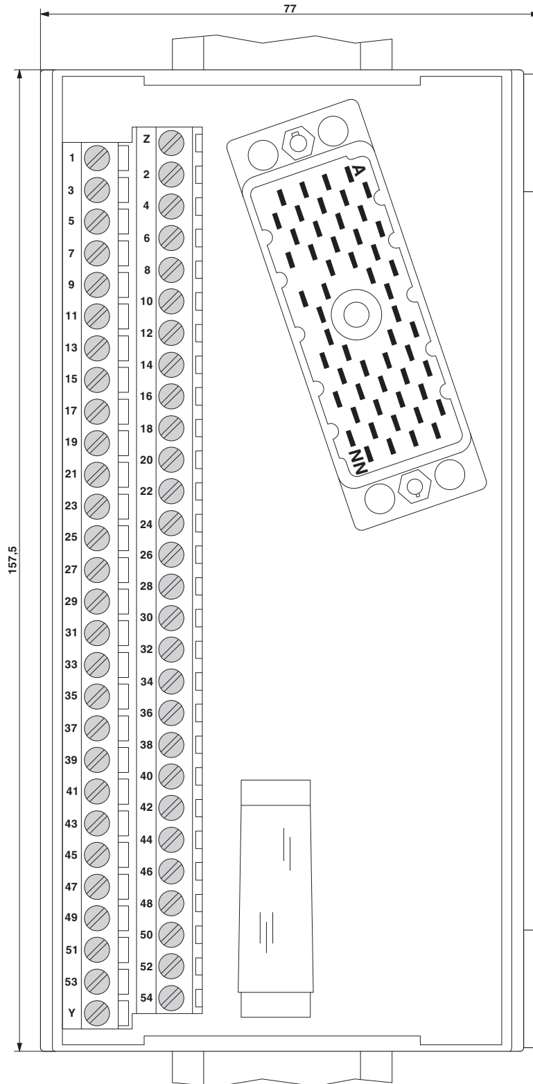
Dimensional drawing
