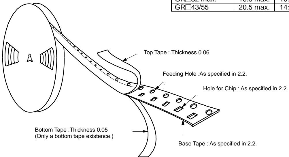
Fig.3 Taping Diagram
