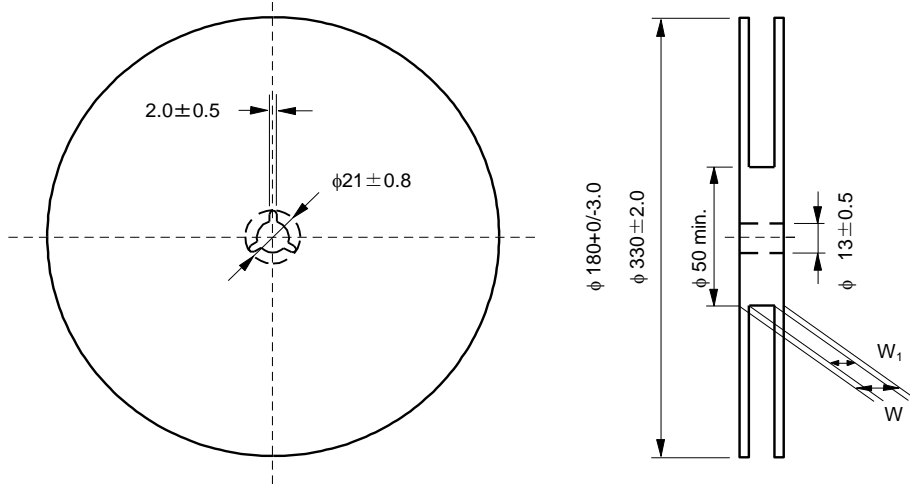
Fig.3 Taping Diagram
