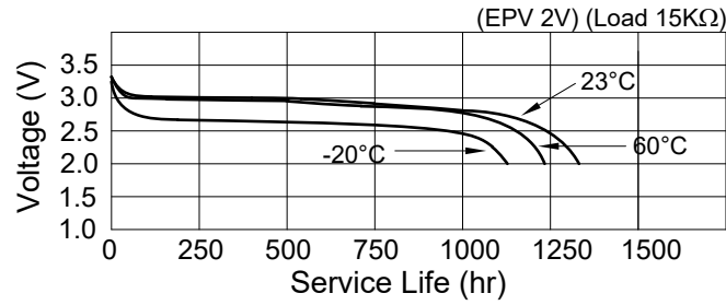
Figure 4. Temperature Characteristics
