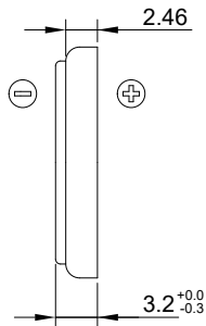
Figure 7. SCR2032/726 Mechanical Layout
