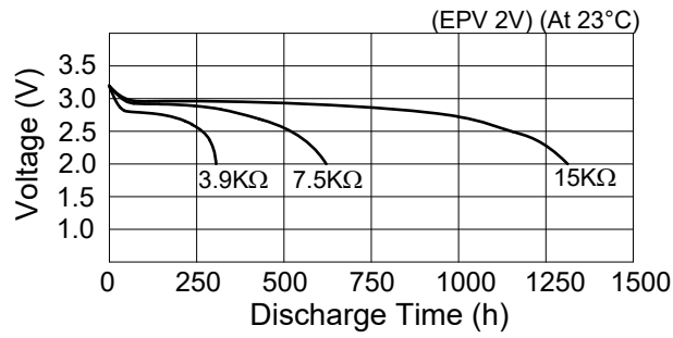
Figure 1. Discharge Characteristics
