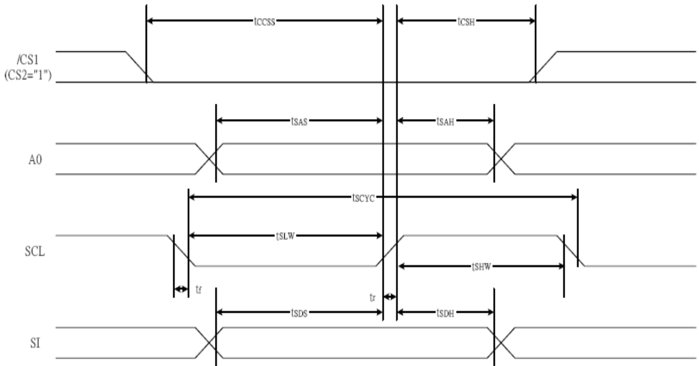
SERIAL INTERFACE(4-Line Interface)
