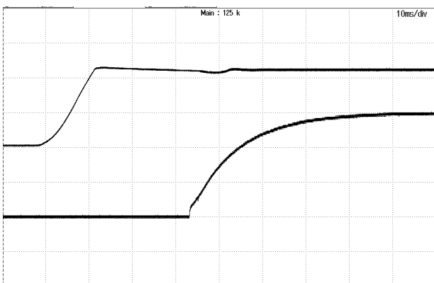
Figure 5: Turn-on transient at zero load current (20ms/div). Top Trace: Vout; 5V/div; Bottom Trace: input voltage: 50V/div.
