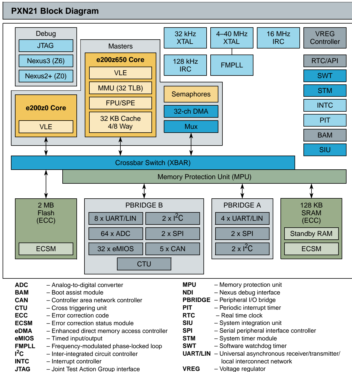
Figure 2. PXN21 Block Diagram
