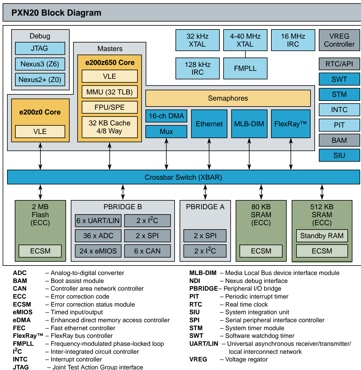
Figure 1. PXN20 Block Diagram
