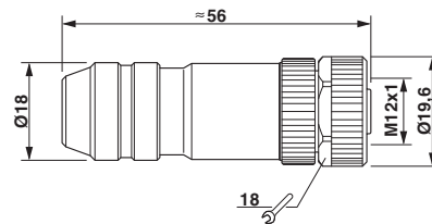
M12 x 1 socket, straight, shielded
