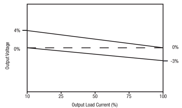
NXJ1S1215MC
