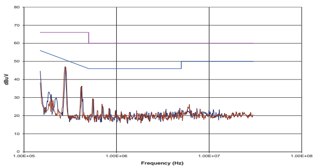
NXJ1S0505MC
