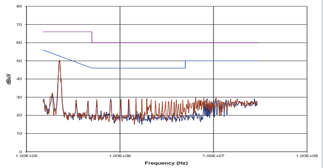
NXJ1S1205MC
