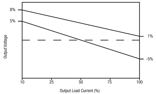
NXJ1S1205MC
