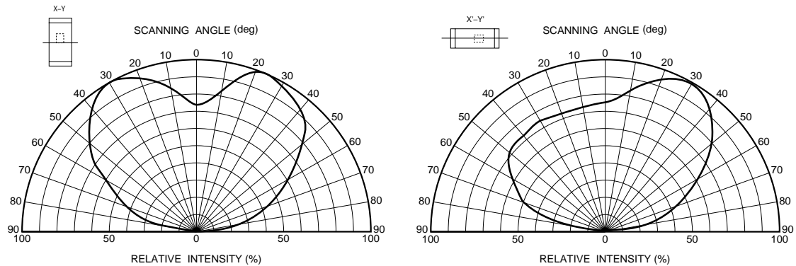
Fig.1 Directional pattern
