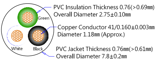
SJT 18AWGx3c 截面圖 (Wire Cross-Section)
