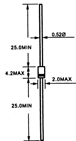
Dimensions in millimeters
