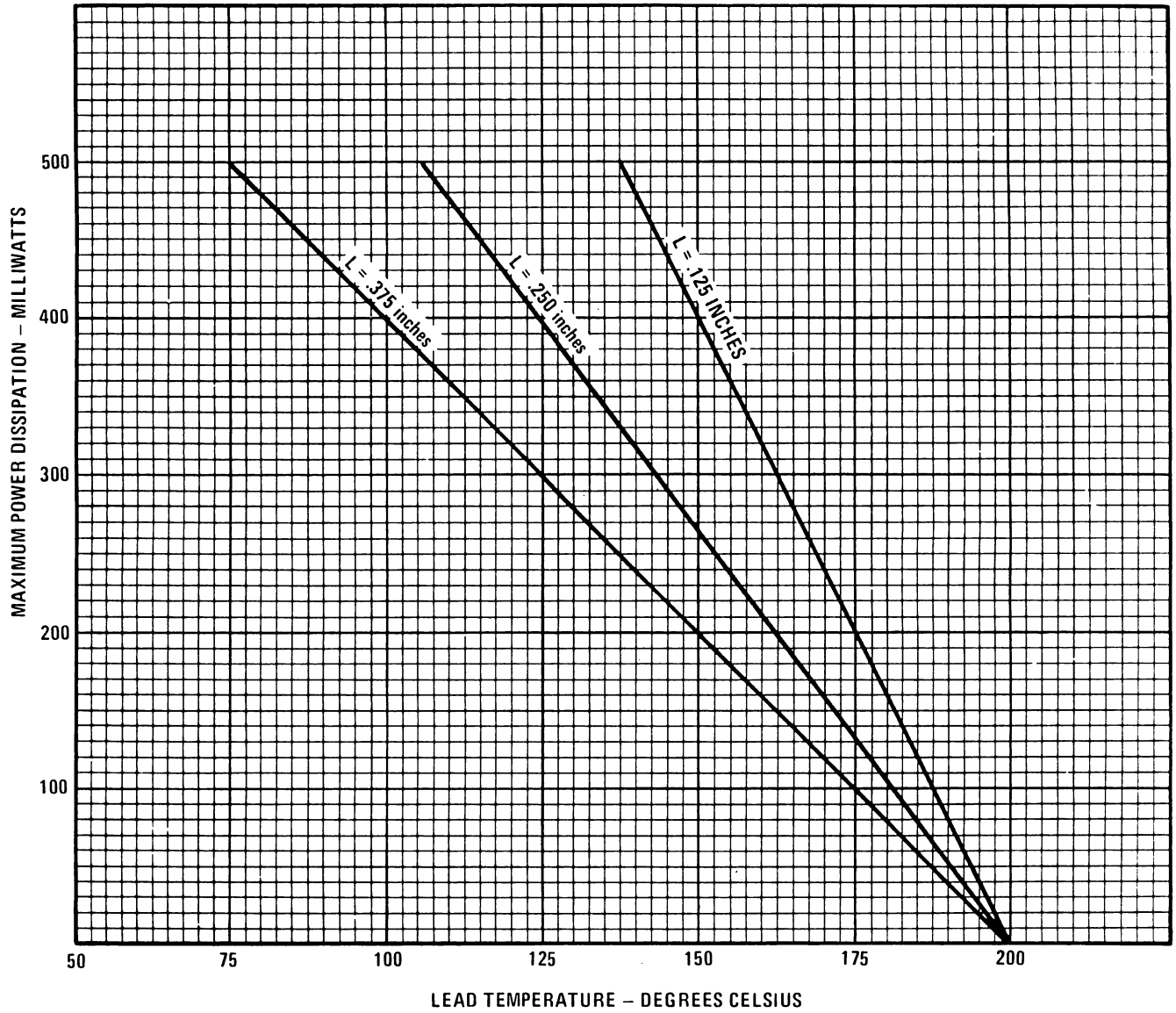
FIGURE 2. MAXIMUM POWER VS. LEAD TEMPERATURE
