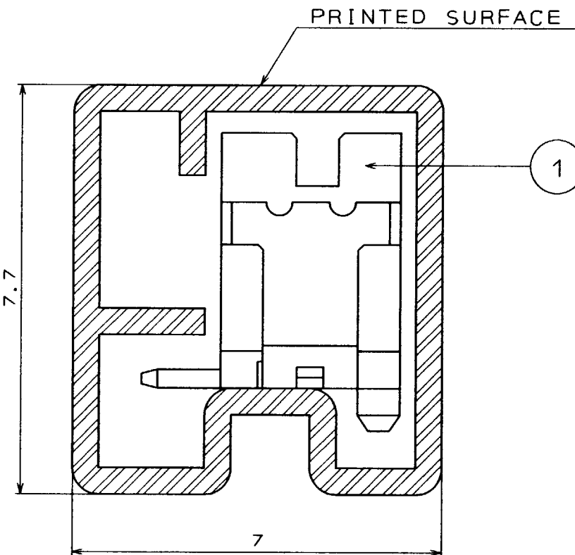
A-A SECTION(10/1)
