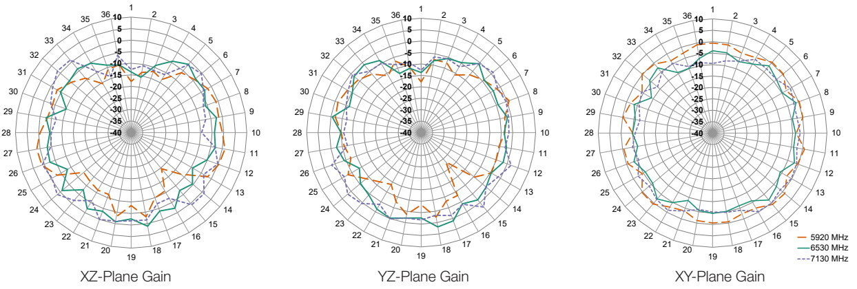
Figure 17. Radiation Patterns for the ANT-W63-WRT Series Antenna at Center of Ground Plane
