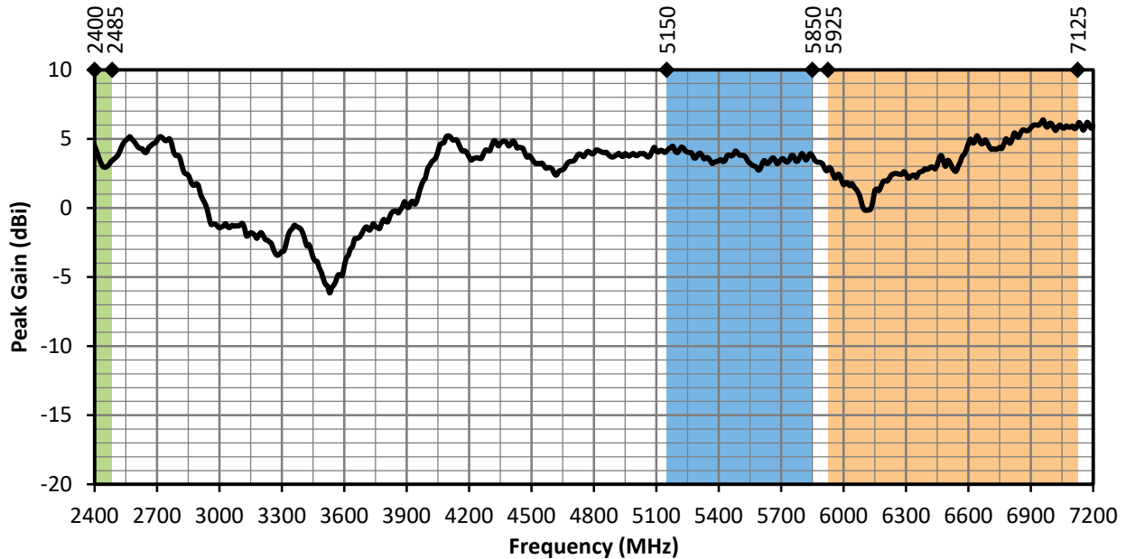
Figure 14. ANT-W63-WRT Antenna Peak Gain at Center of Ground Plane
