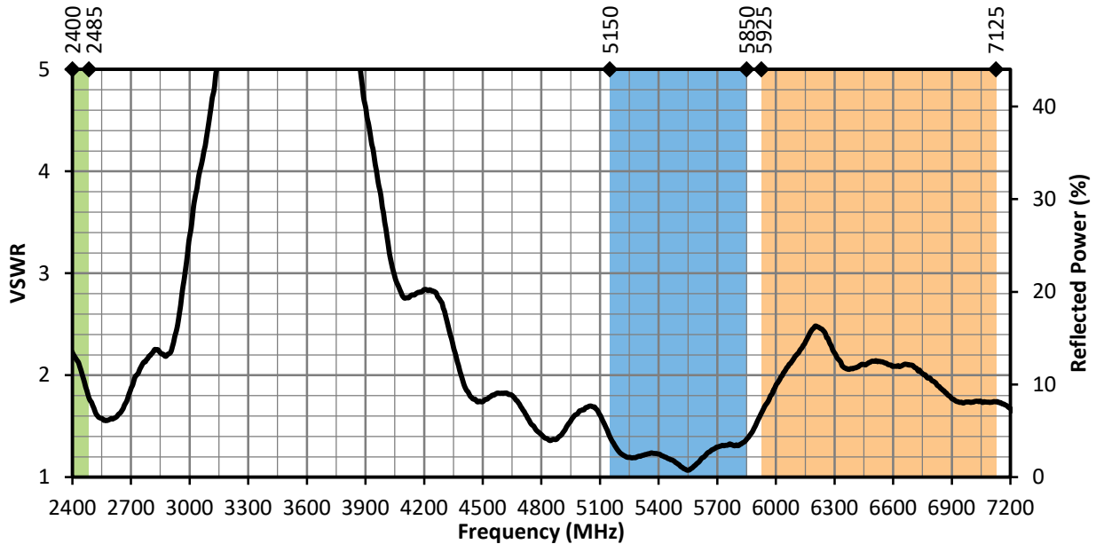
Figure 5. ANT-W63-WRT VSWR, Free Space
