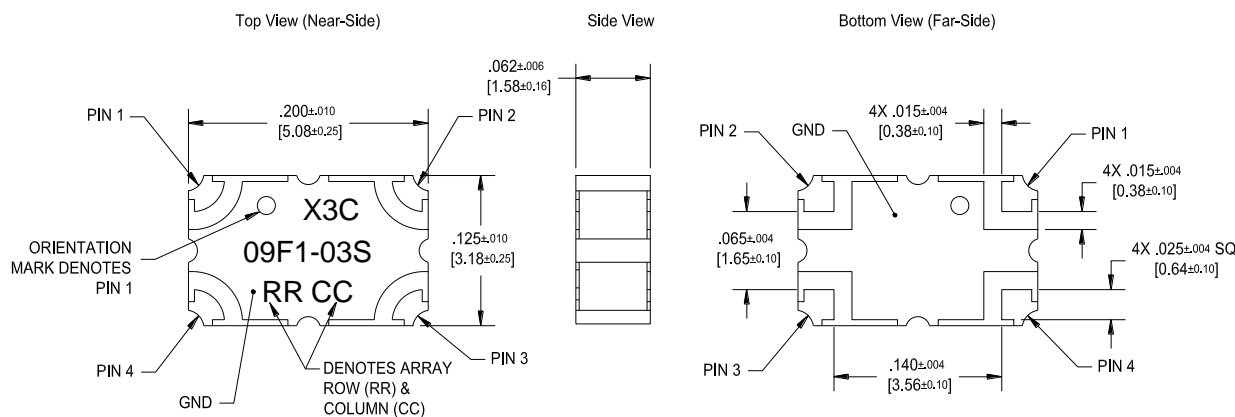
Dimensions are in Inches [Millimeters] X3C09F1-03S Mechanical Outline
