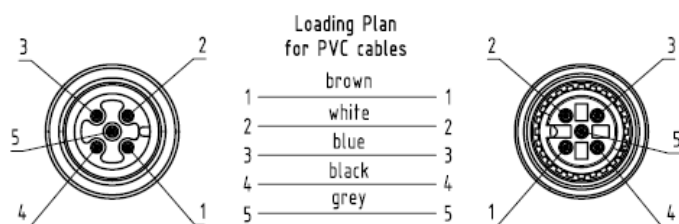
Male and Female 5-pole
