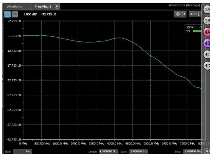
Figure 5: PV1 frequency-domain gain response
