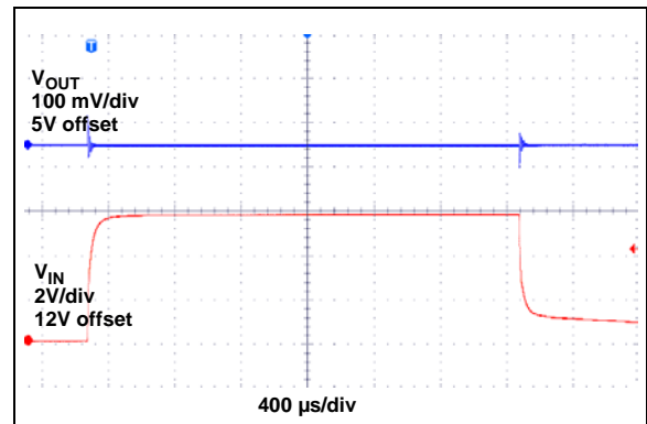
FIGURE 2-42: Line Transient Response (12V to 18V).
