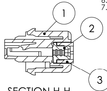
SECTION H-H
